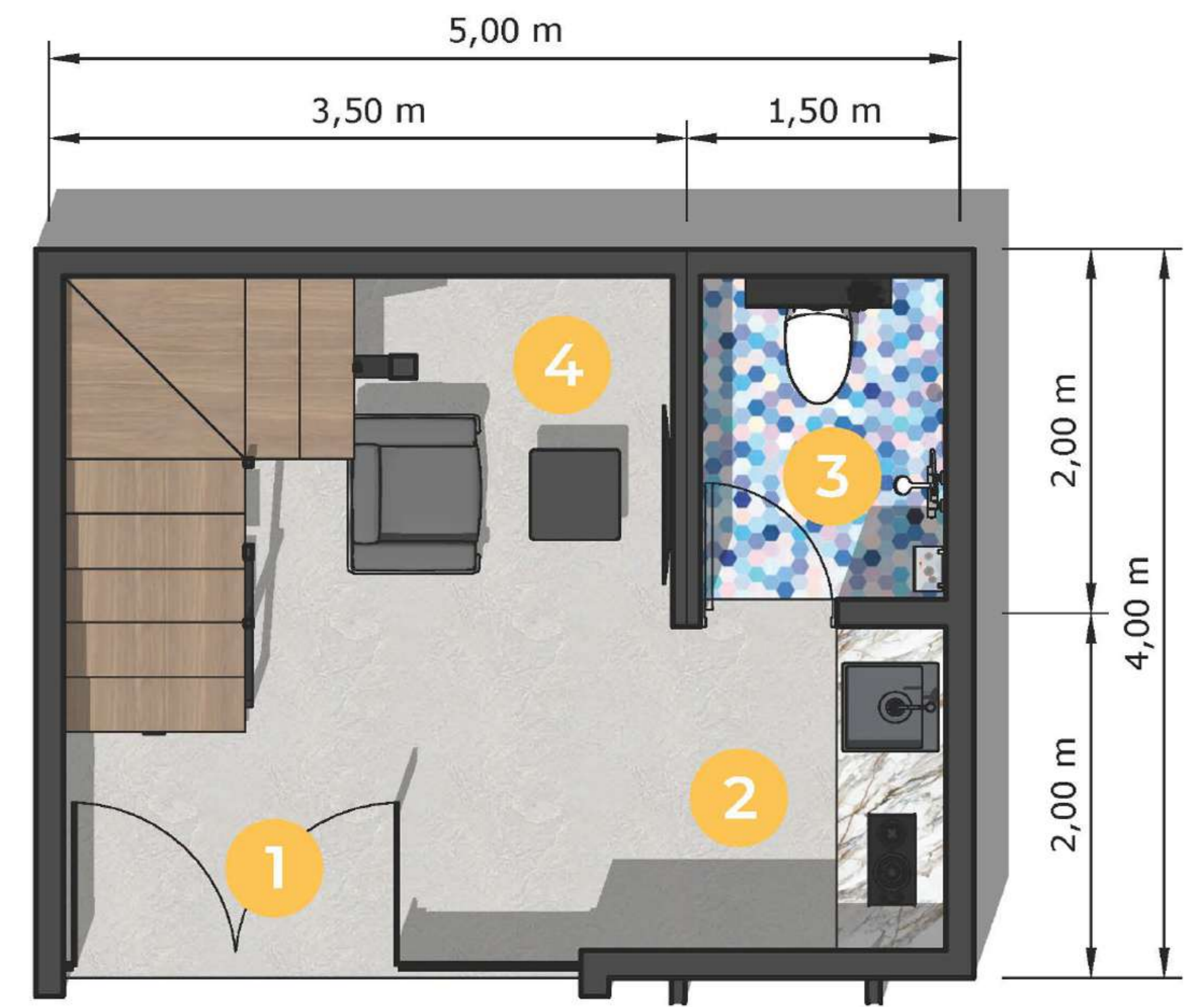
DENAH LANTAI 1
