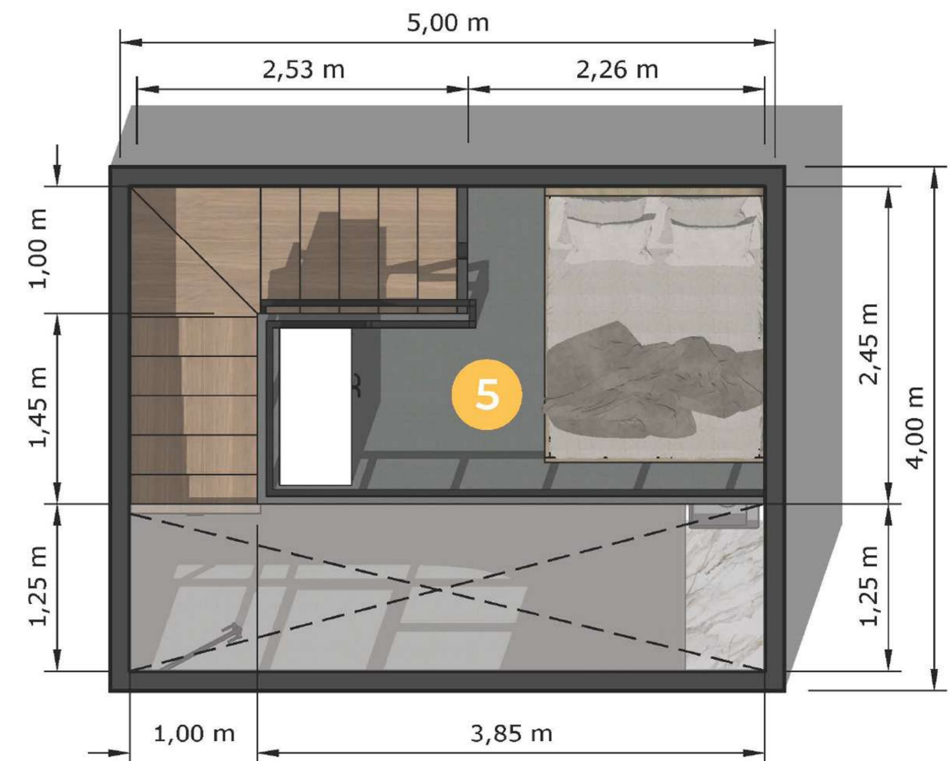
DENAH MEZZANINE
